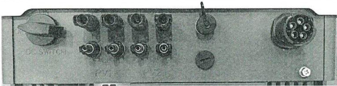
DC SWITCH, PV CONNECTOS, COM PORT AND AC OUTPUT PORT
