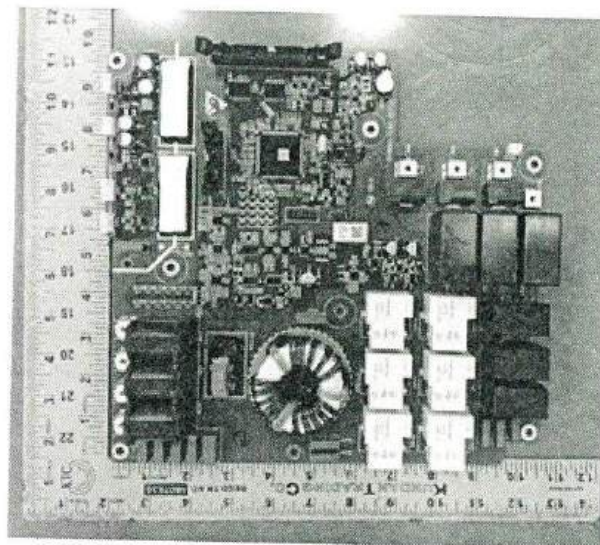
PCB BOARD COMPONENT SIDE VIEW
