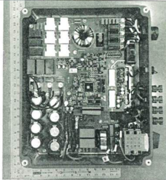
INTERNAL VIEW
