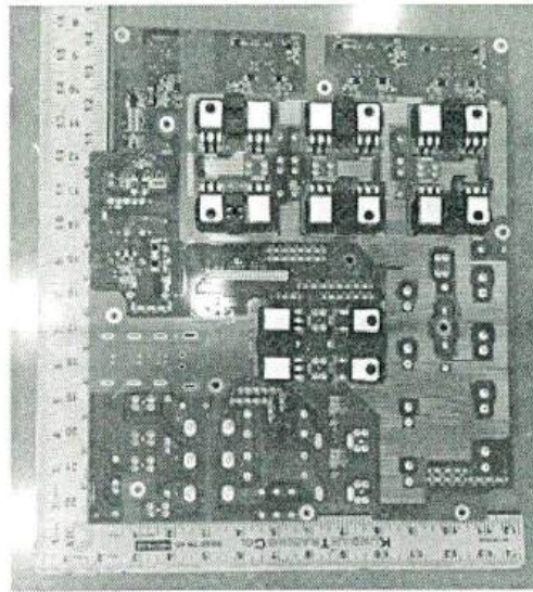
PCB BOARD SOLDER SIDE VIEW
