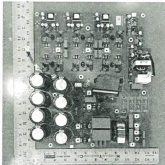
PCB BOARD COMPONENT SIDE VIEW
