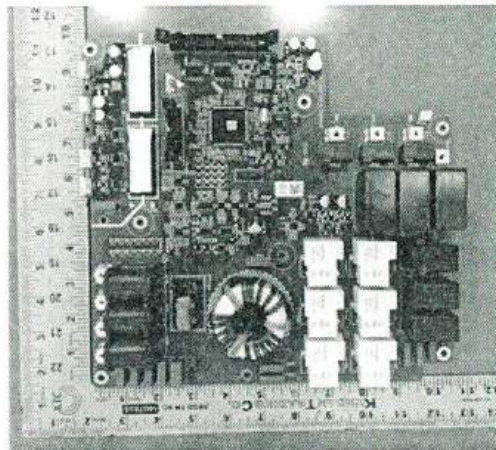
PCB BOARD COMPONENT SIDE VIEW
